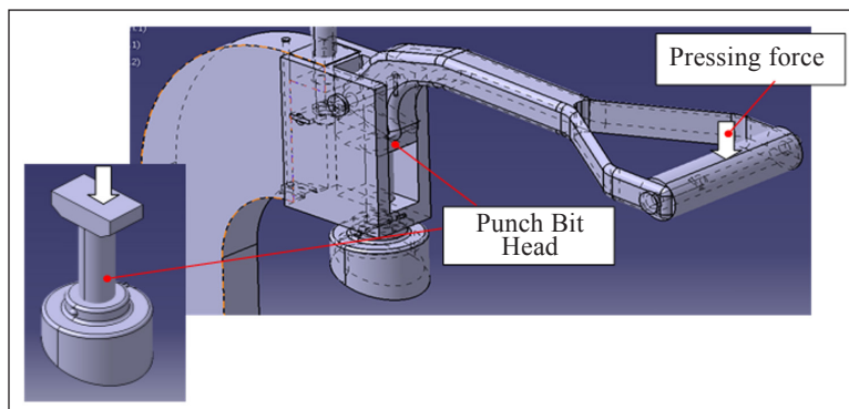
Figure 13. Punch bit head
