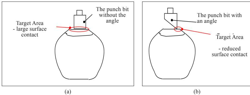
Figure 5. The effective area of a punch bit design
