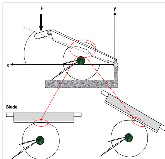
Figure 11. The blade angle during cutting process
