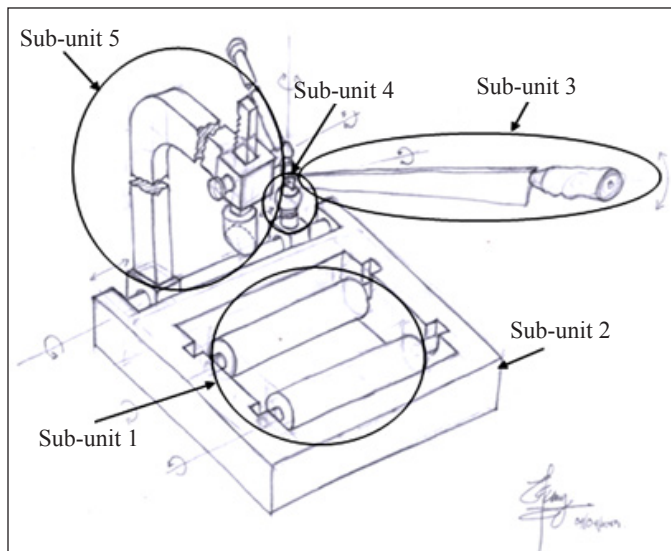
Figure 1. Preliminary design for five (5) sub-units
