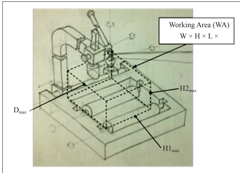
Figure 3. Young coconut processing apparatus's working area
