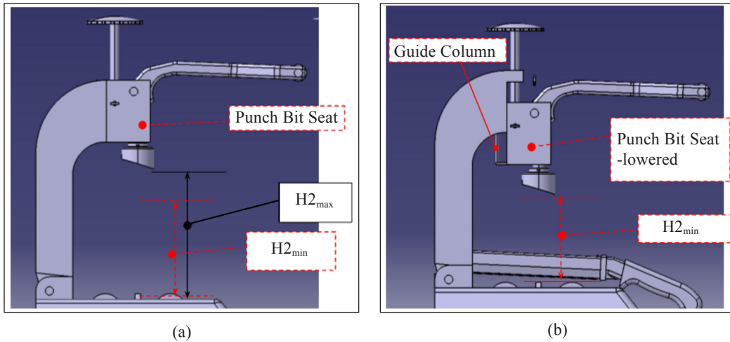
Figure 6. The different position of the punch bit seat
