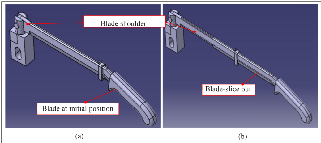
Figure 10. Slicing movement of the blade with respect to its holder
