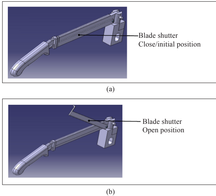
Figure 8. Blade safety mechanism
