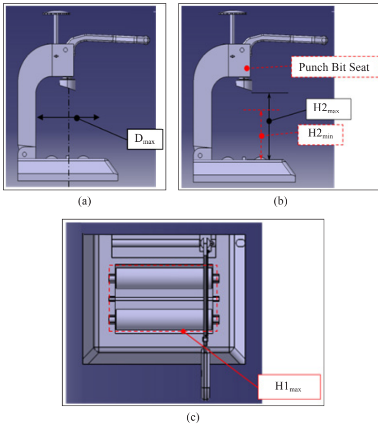
Figure 4. Young coconut apparatus working area terms definition
